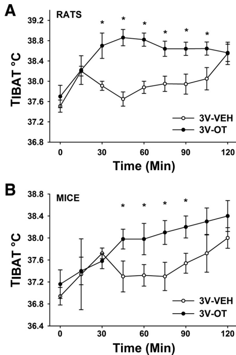
Fig. 7. Effects of 3V OT administration on interscapular brown adipose tissue temperature ( T_{IBAT} ) in rats and mice. A : T_{IBAT} in rats that received acute 3V injections of OT ( 5 \mu\text{g}/\mu\text{l} ) or vehicle ( n = 10/\text{group} ). B : T_{IBAT} in mice that received an acute 3V injection of OT ( 5 \mu\text{g}/\mu\text{l} ; n = 5/\text{group} ). Values are means \pm SE. *P < 0.05 , OT vs. vehicle.
