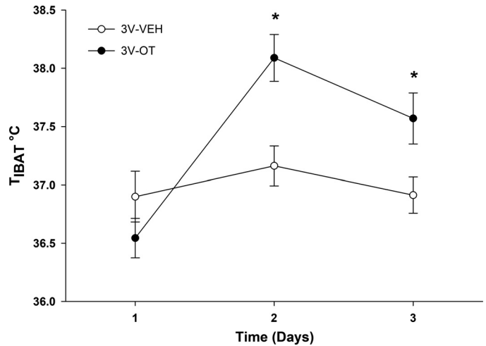
Fig. 9. Effects of chronic 3V OT administration on T_{IBAT} in DIO Long-Evans rats. T_{IBAT} was measured daily during 72-h infusions of OT ( 16 \text{ nmol}/\text{day} ) or vehicle in 3-h-fasted rats ( n = 8 – 10/\text{group} ). Values are means \pm SE. *P < 0.05 , OT vs. vehicle.
